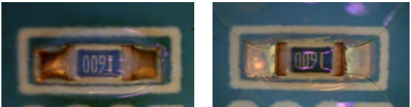
Figure 6. Thermal shock reliability test on populated boards: LM1 (left), LM2 (right)
